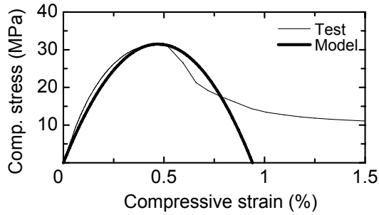
Fig.1 Stress - strain curves
